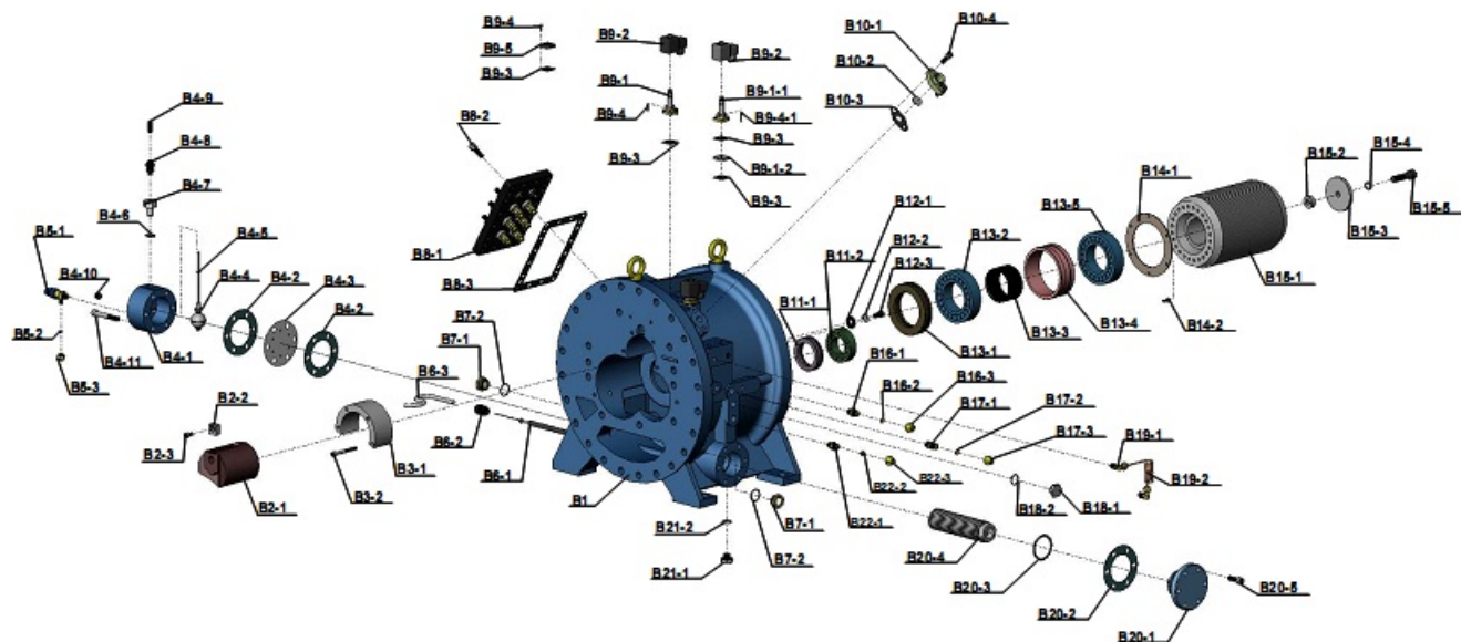
RC2-170~620 Except 180&610 B - Compression Casing
